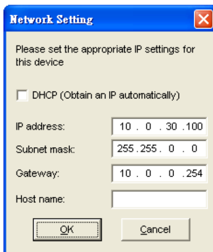
Fig. 2. IP Settings using DeviceView Utility software
